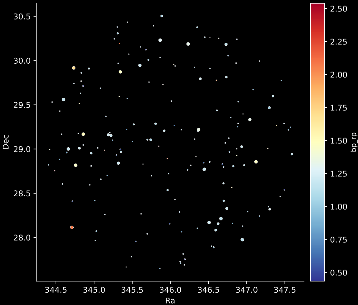
APOGEE DR17 Field: [048+44_MGA] Stars: 172
