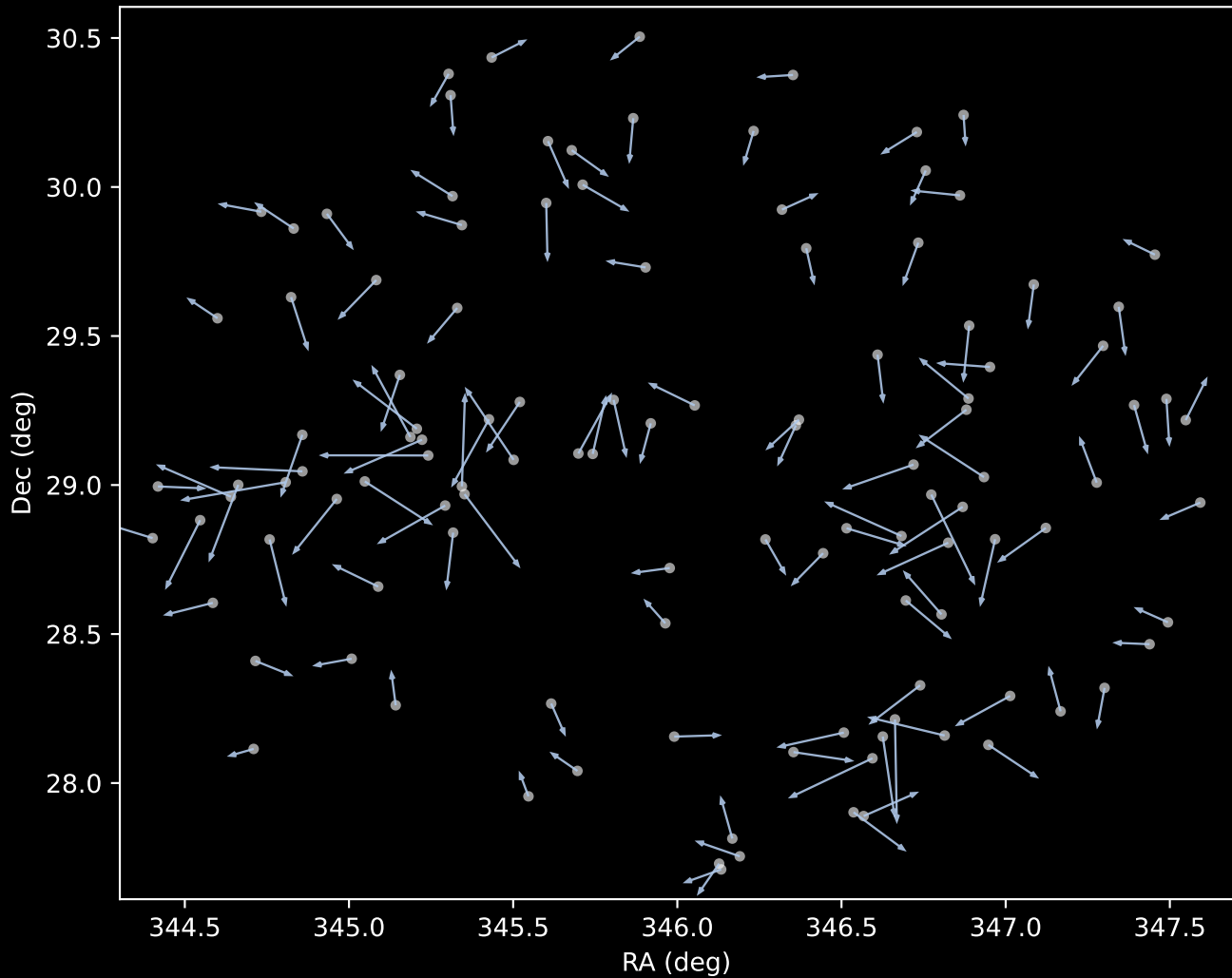
APOGEE DR17 Cluster 1 Proper Motion Vectors (n=116)
