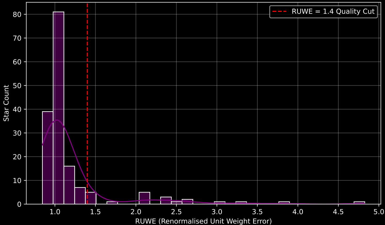
GAPOGEE DR17 Field [048+44_MGA] RUWE Distribution (n= 164)
