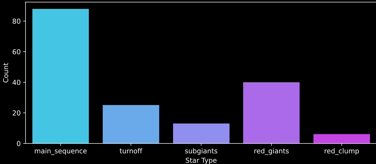
APOGEE DR17 Field: [048+44_MGA] Count plot of Star Type
