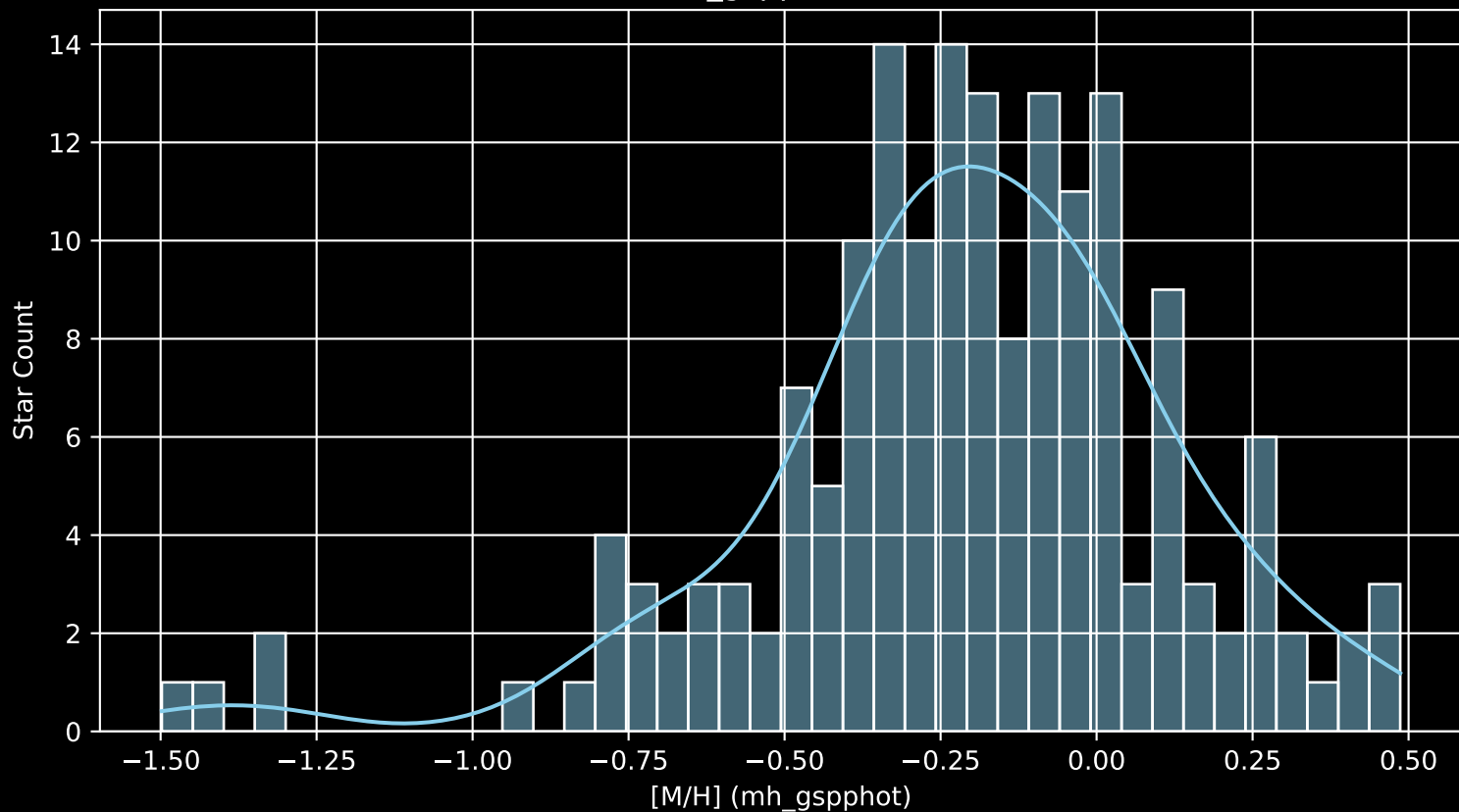
APOGEE DR17 Field: [048+44_MGA [M/H] (mh_gspphot) (n= 172)
