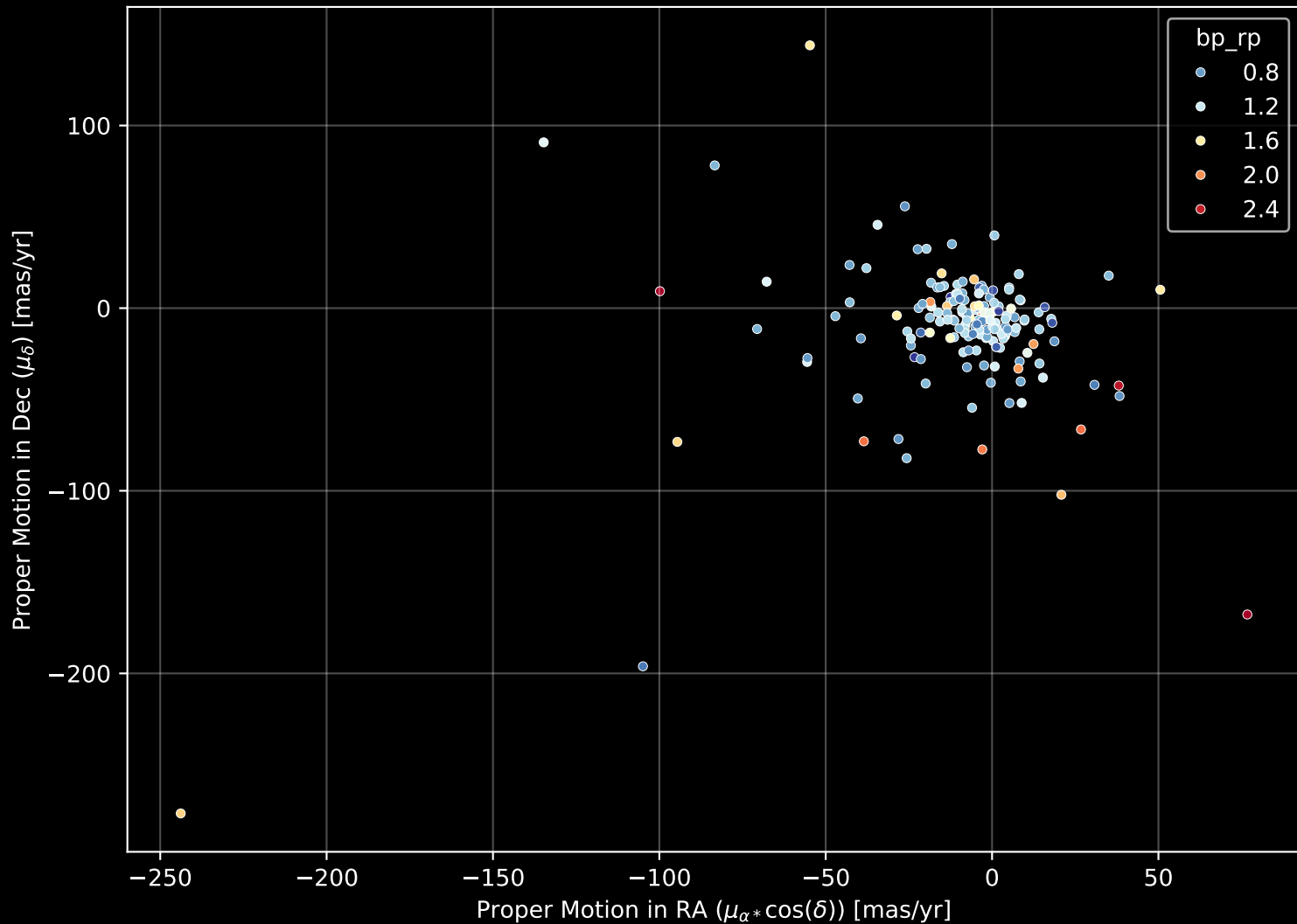
APOGEE DR17 Field: [048+44_MGA] Proper Motion Diagram (n= 172)
