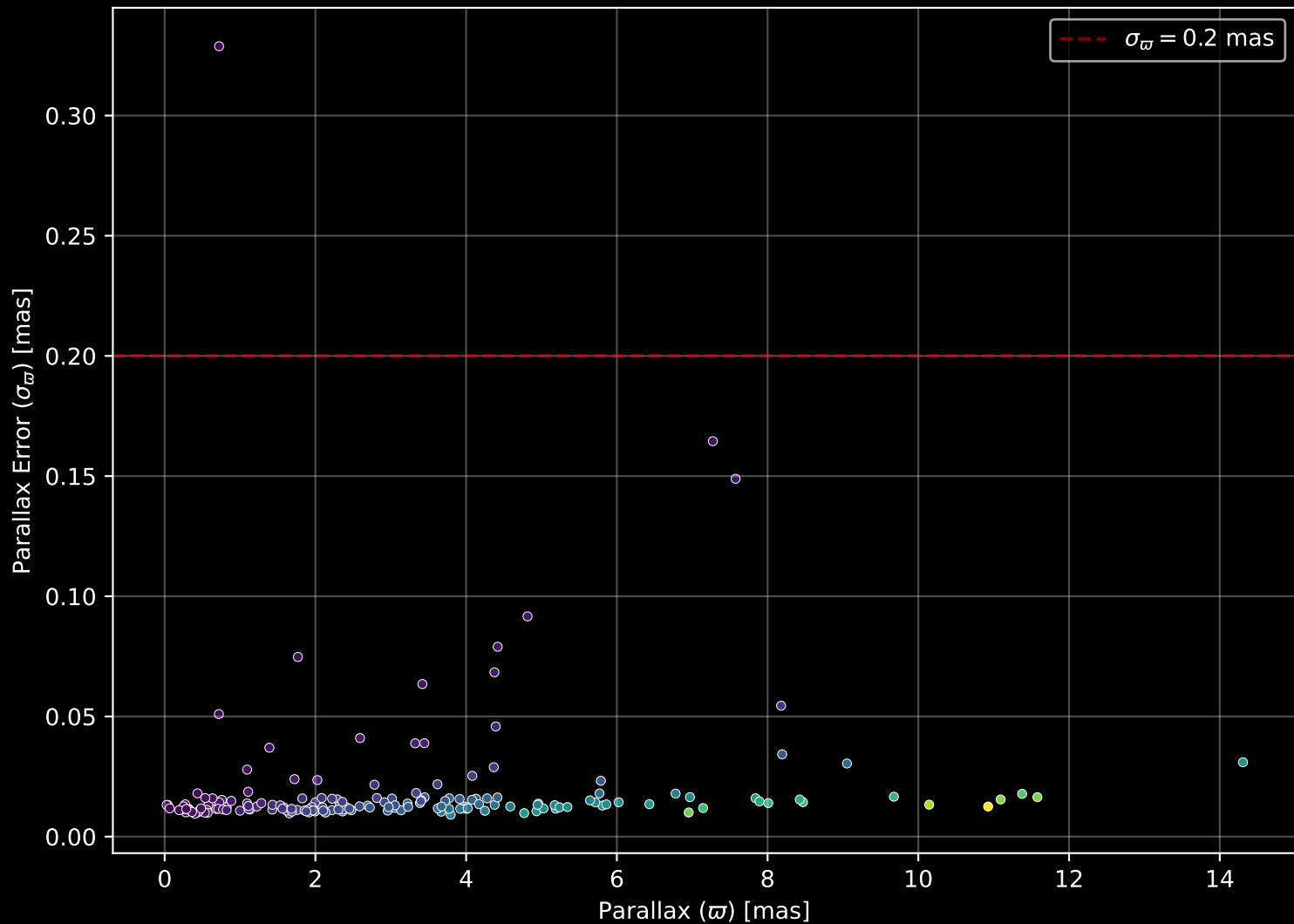
APOGEE DR17 Field: [048+44_MGA] Parallax Quality (n= 172)
